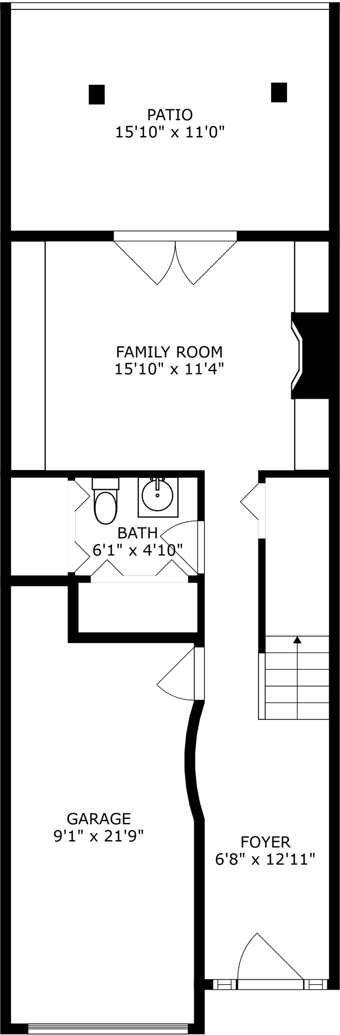
FLOOR 1
