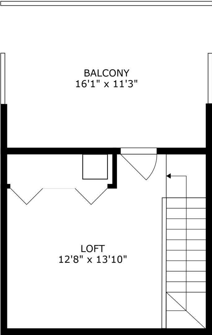
FLOOR 4
