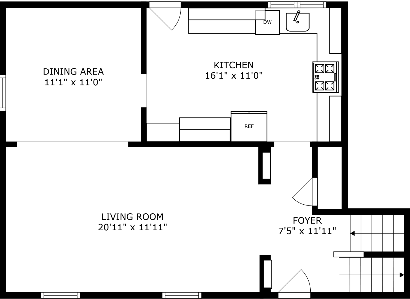
FLOOR 2
