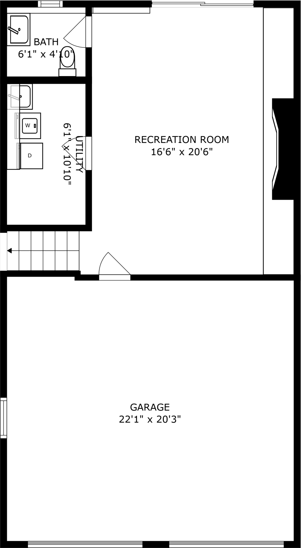
FLOOR 1
