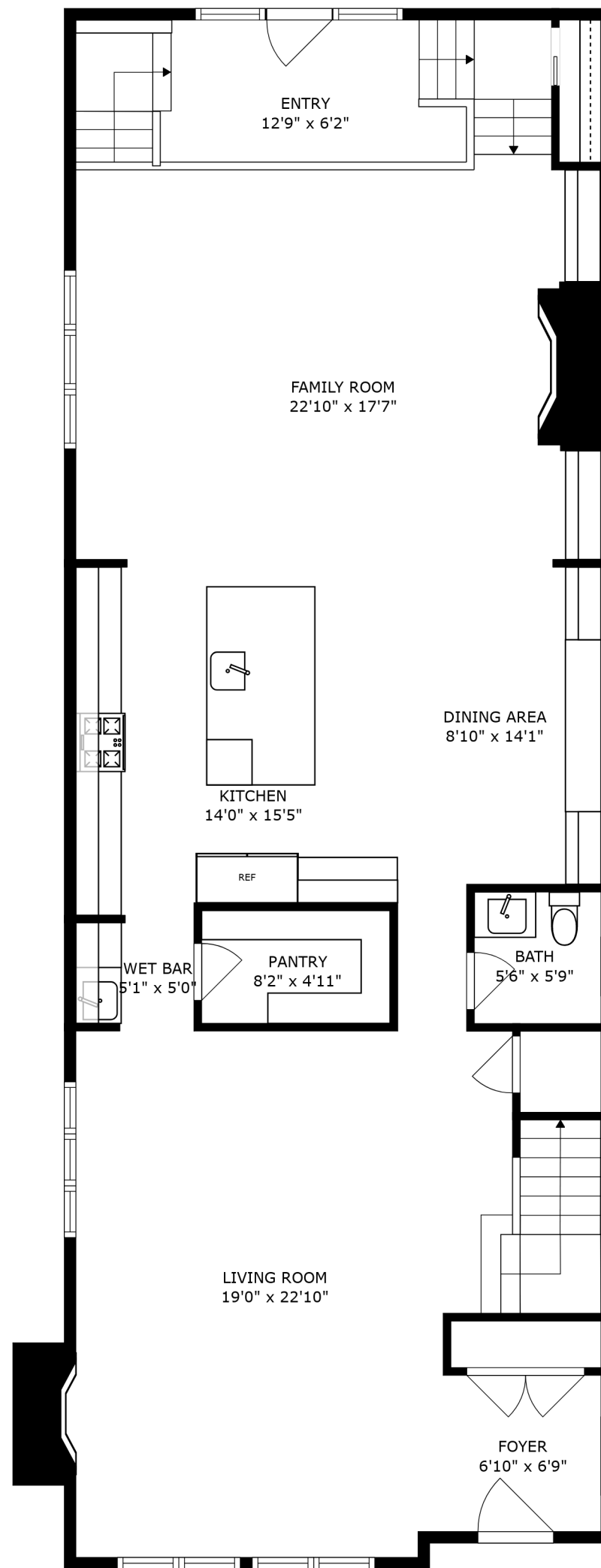
FLOOR 2
