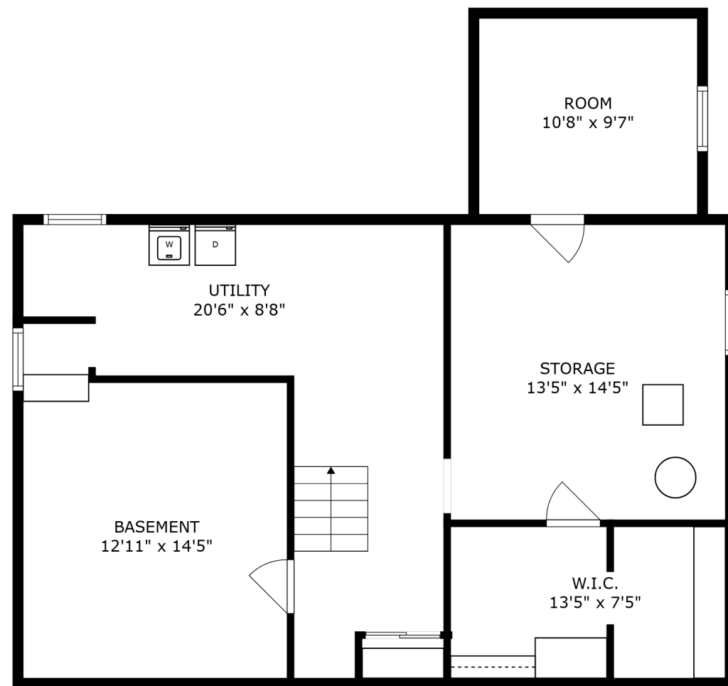
FLOOR 2
