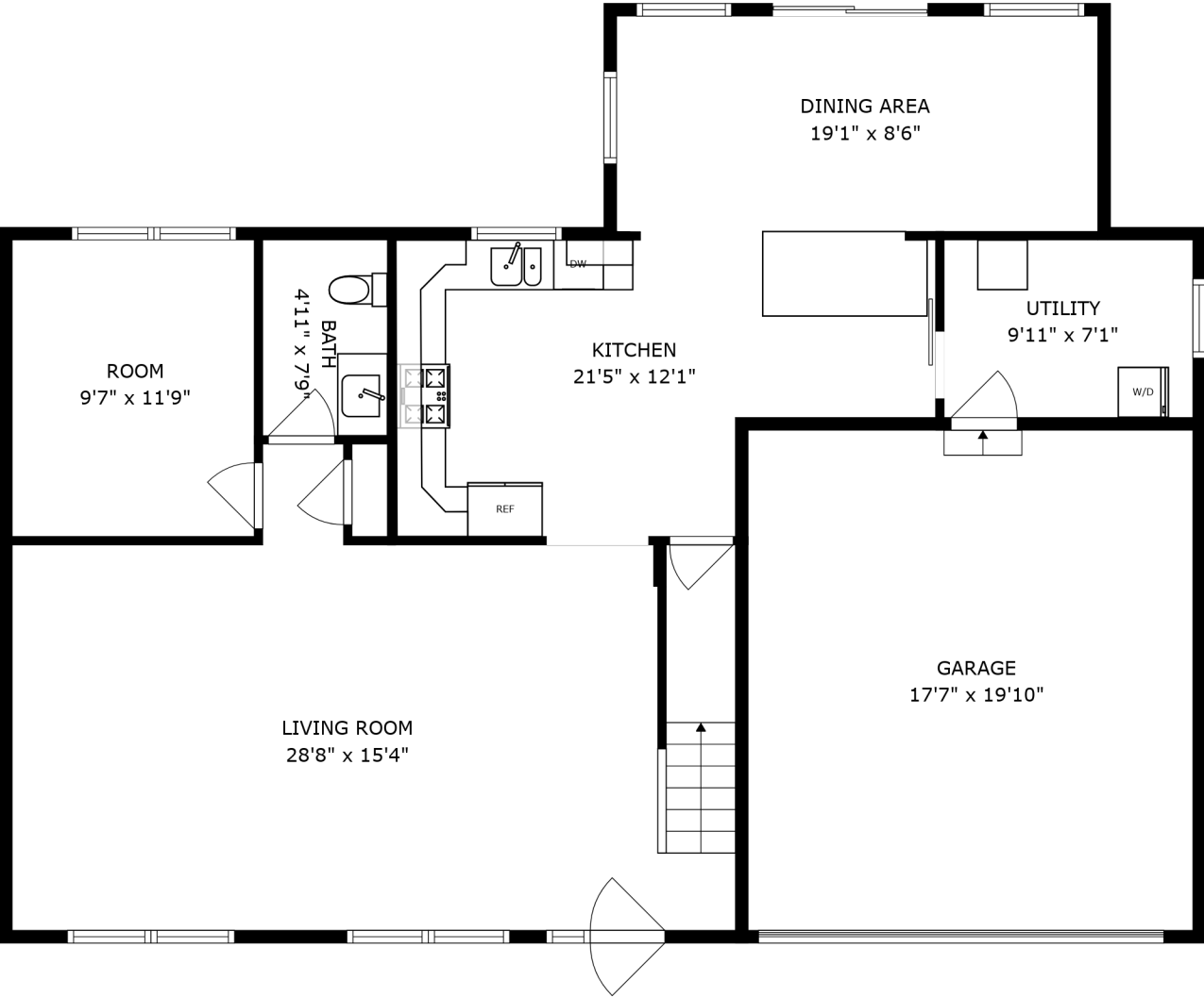
FLOOR 1
