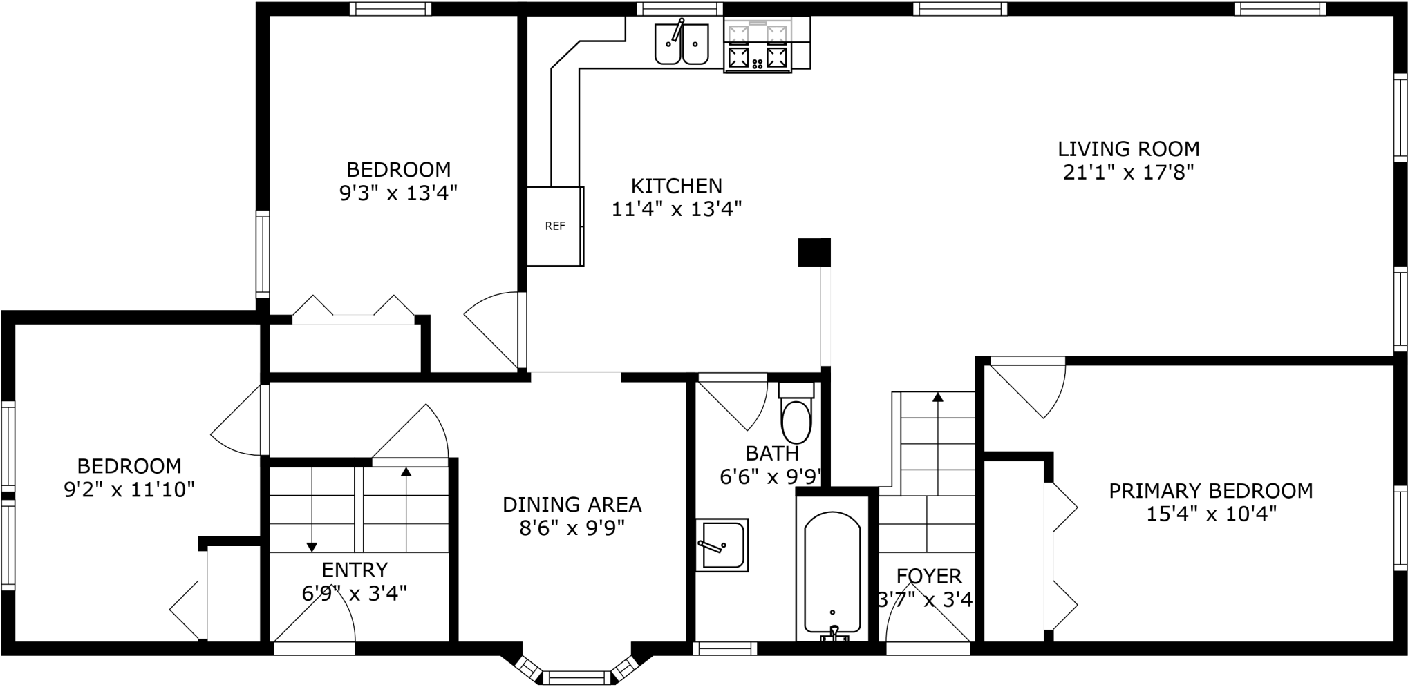
FLOOR 2
