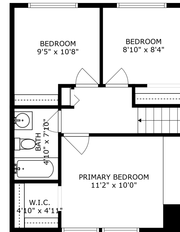
FLOOR 3
