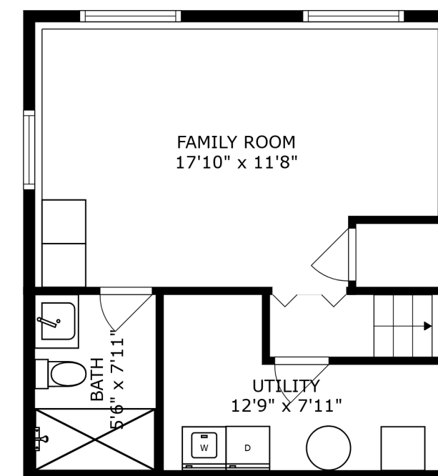
FLOOR 1
