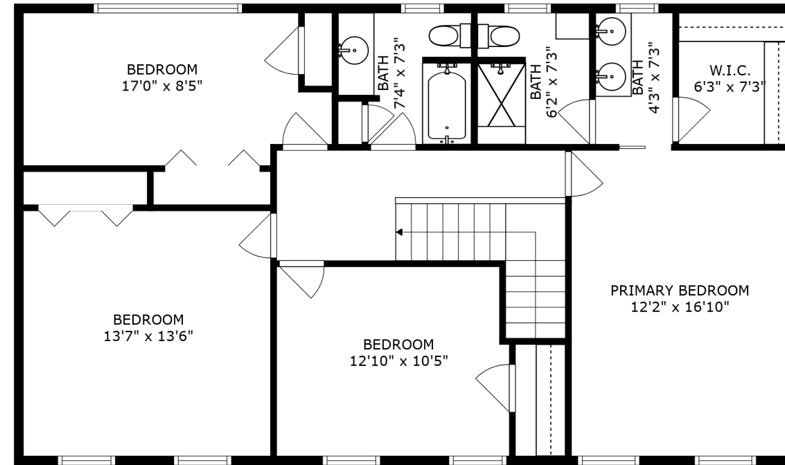
FLOOR 3
