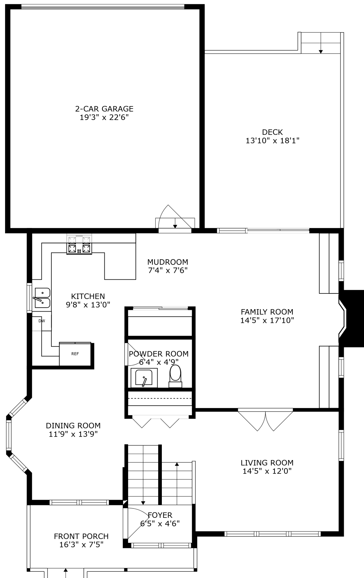
FIRST FLOOR
