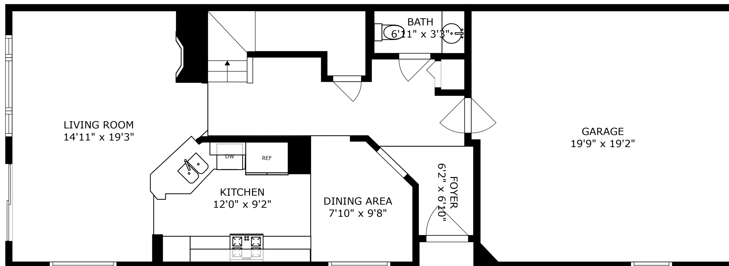
FLOOR 2
