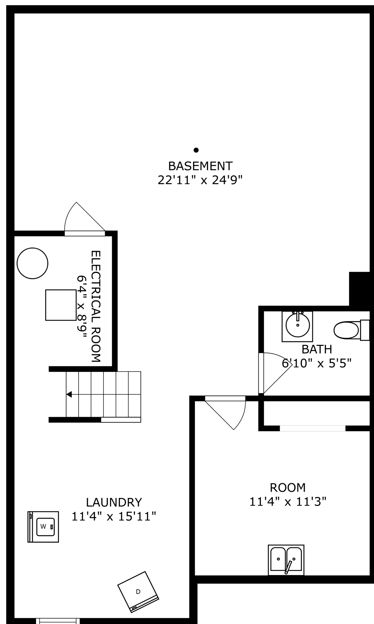
FLOOR 1
