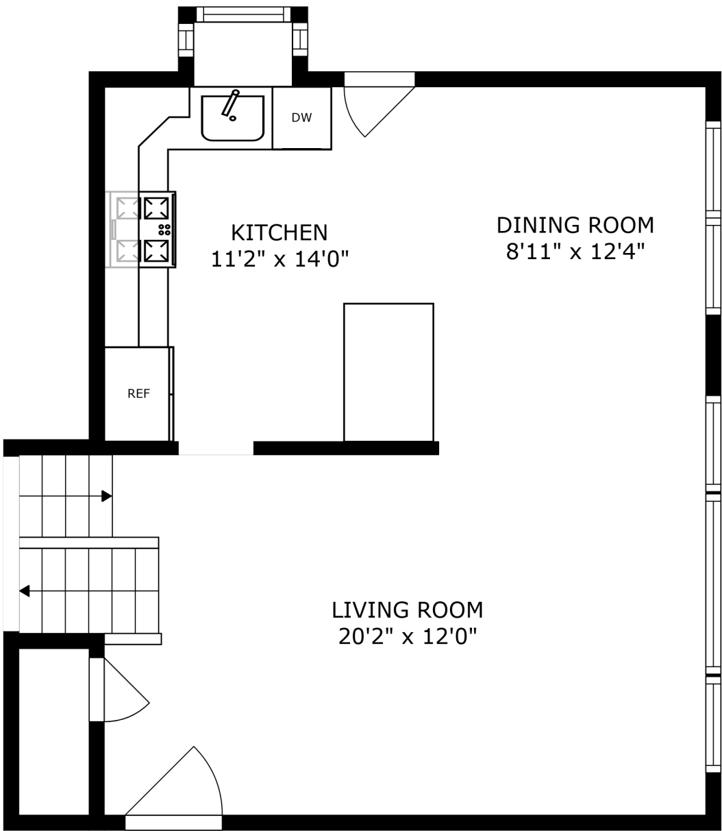
FLOOR 2
