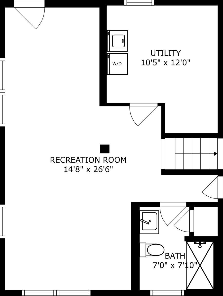
FLOOR 1
