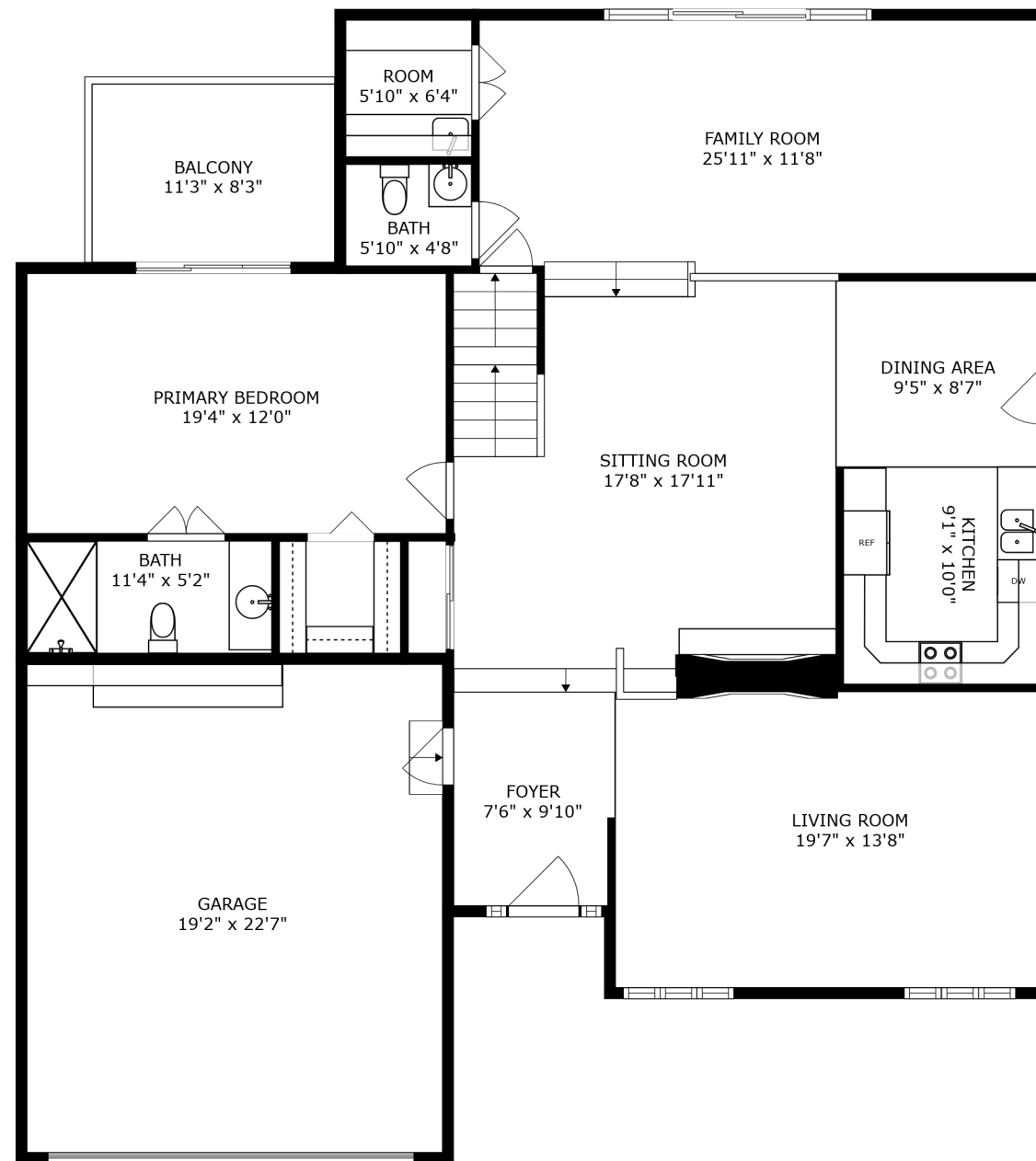
FLOOR 2
