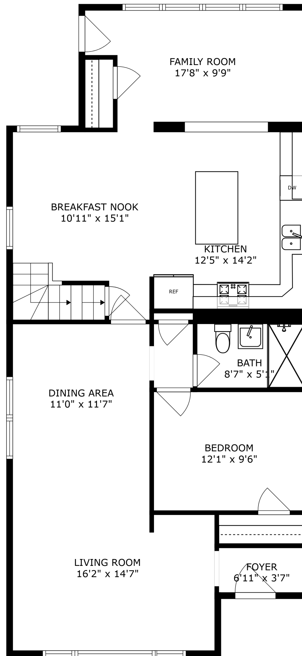
FLOOR 2
