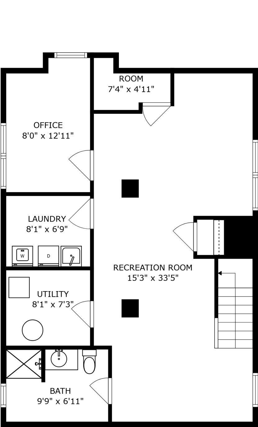
FLOOR 1
