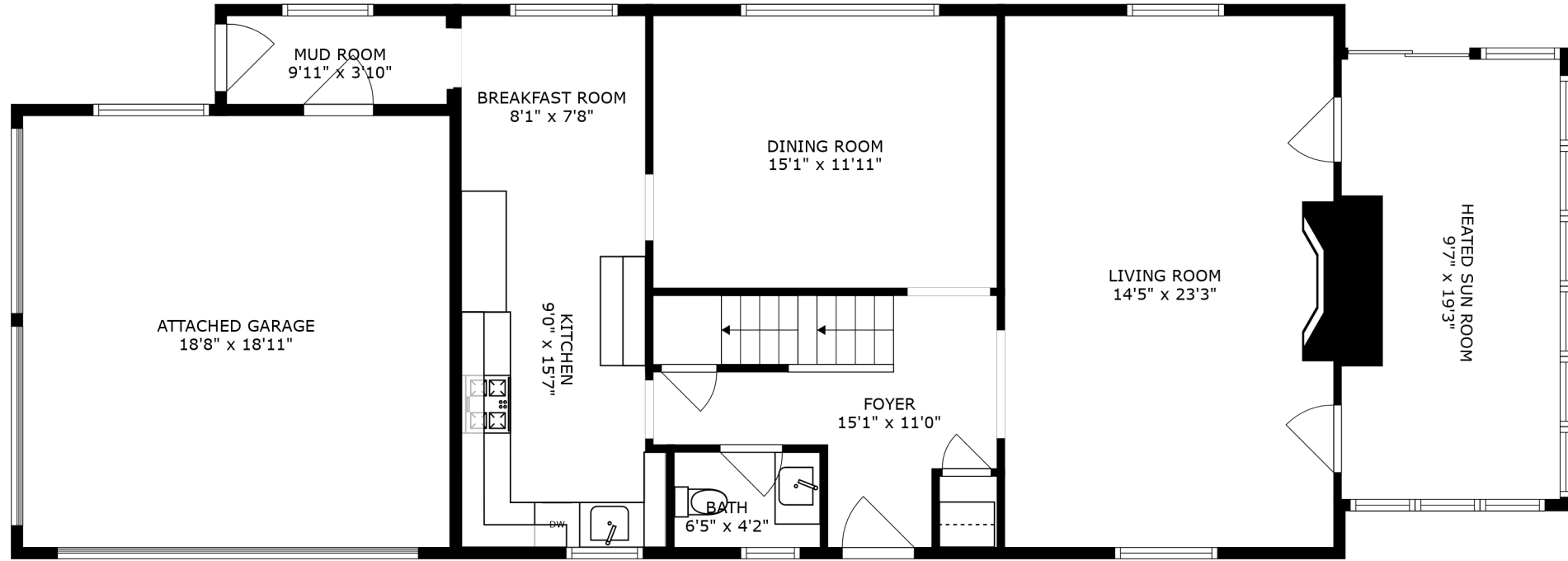
FLOOR 2
