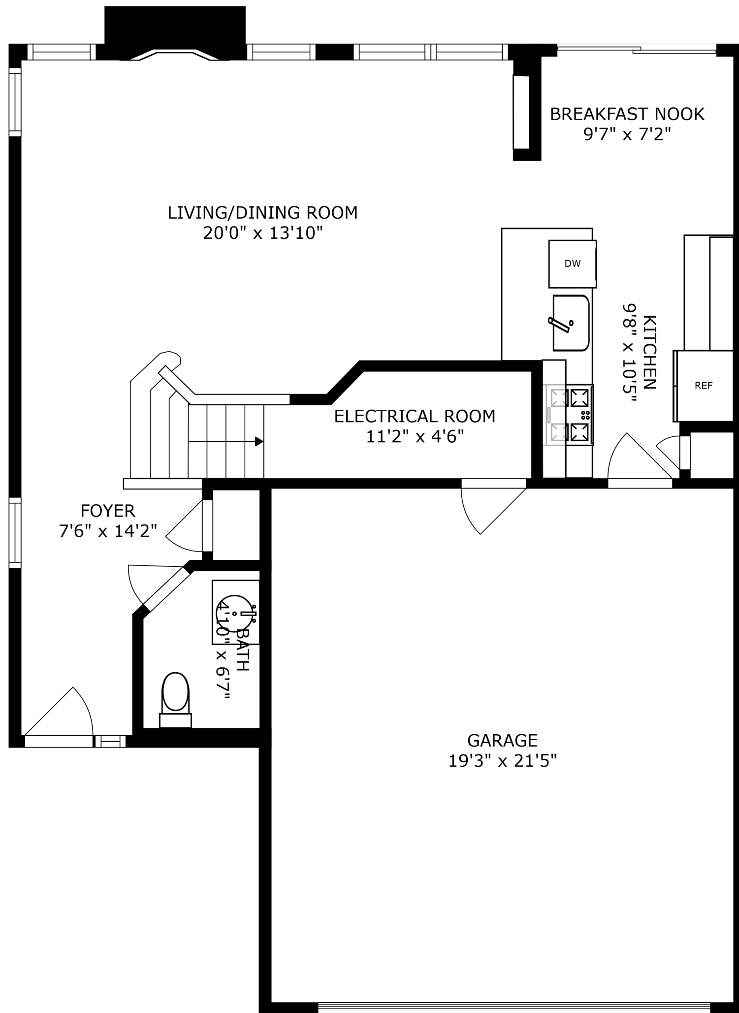
FLOOR 1
