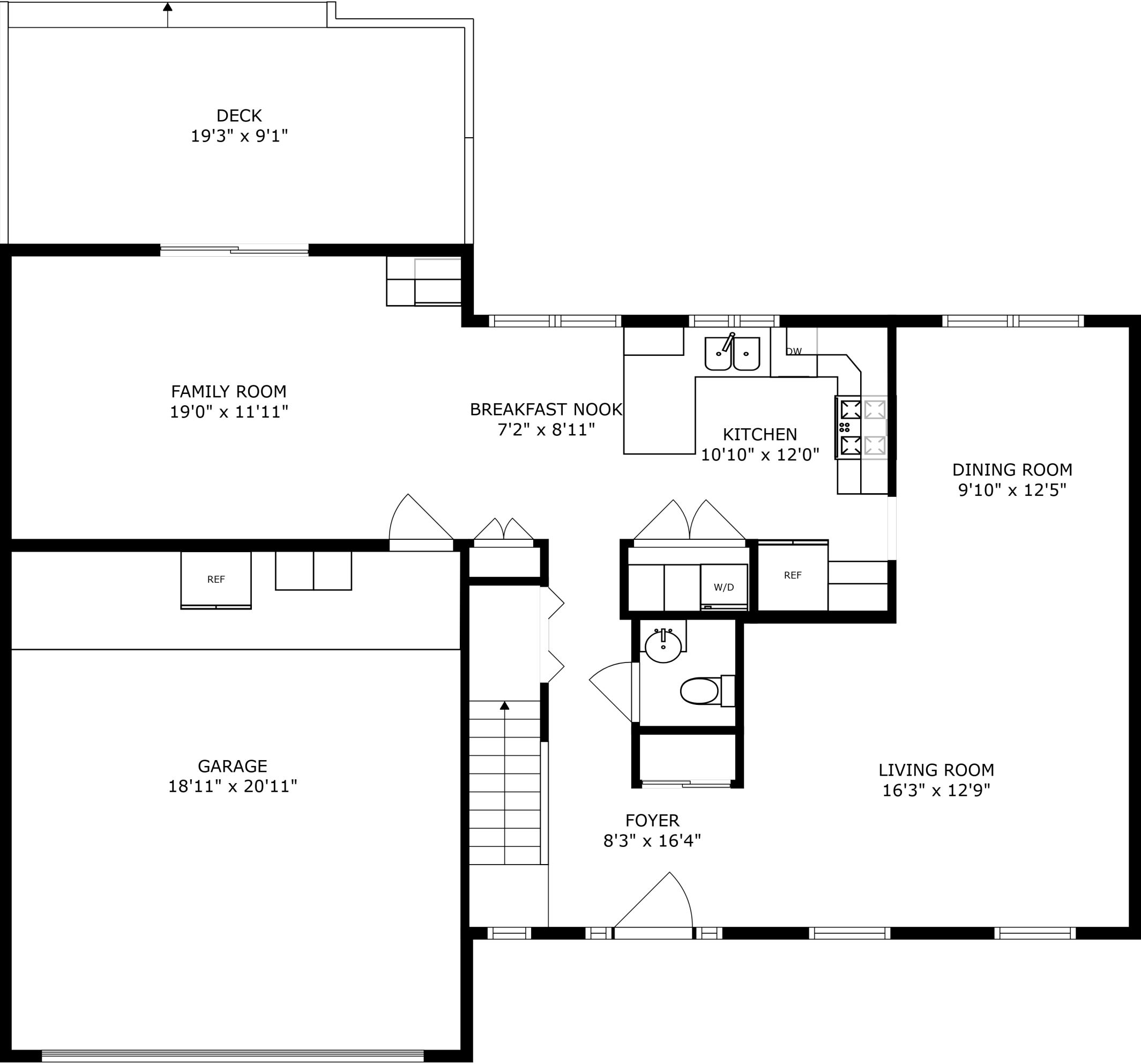
FLOOR 1
