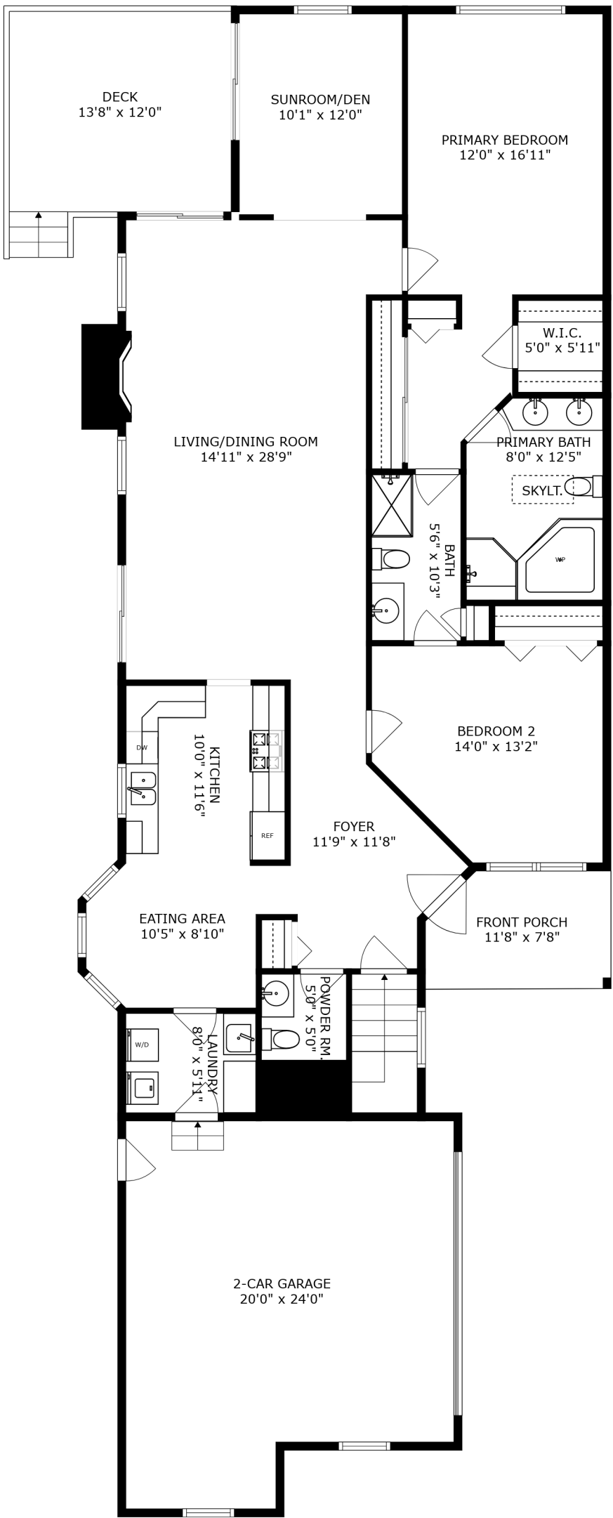
FIRST FLOOR
