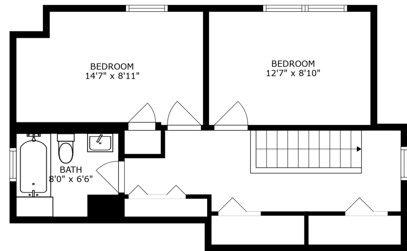
FLOOR 3
