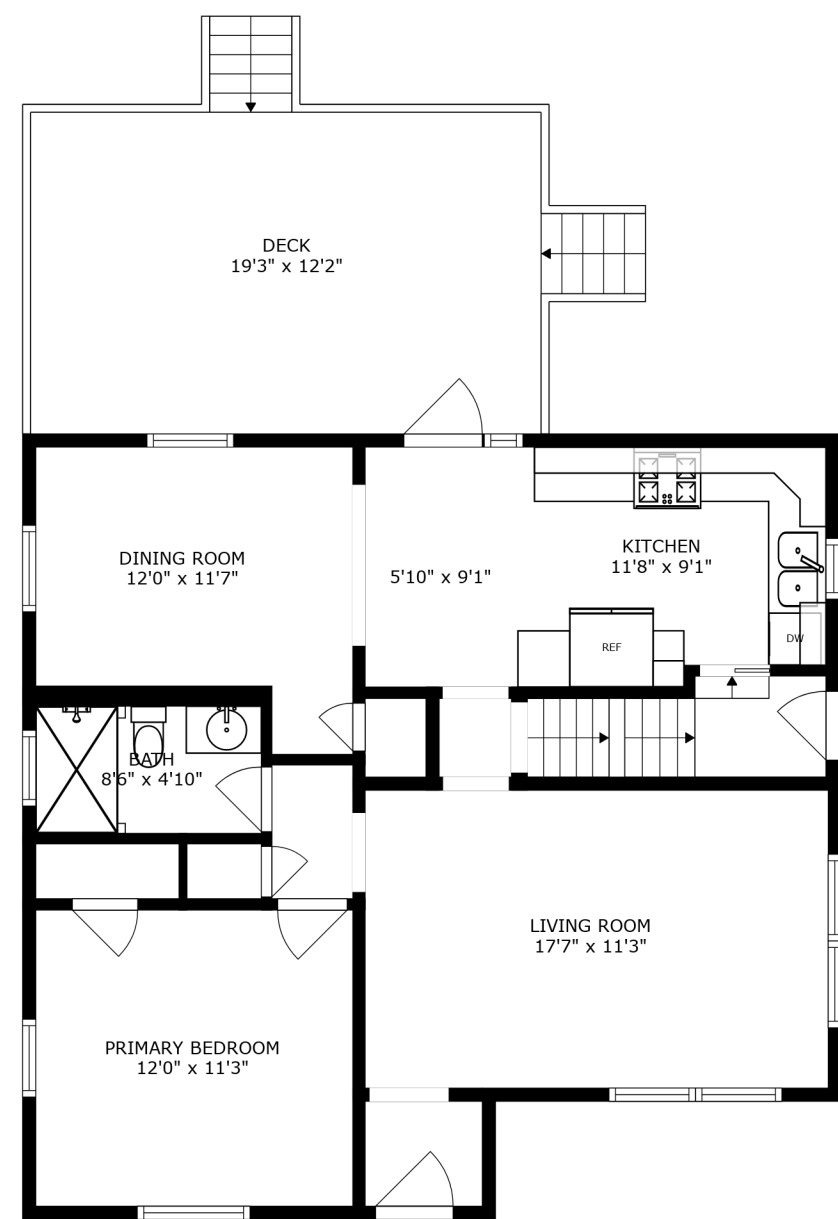
FLOOR 2
