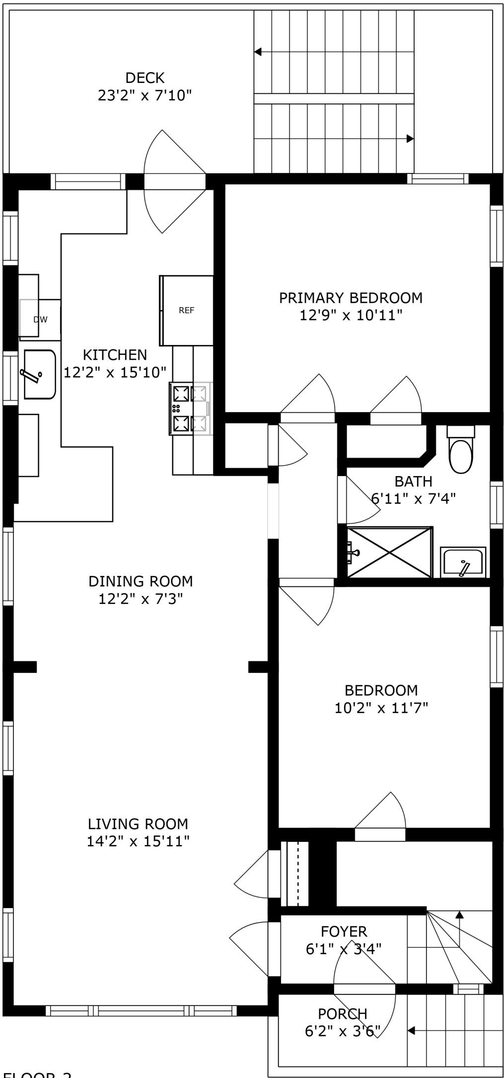
FLOOR 2
