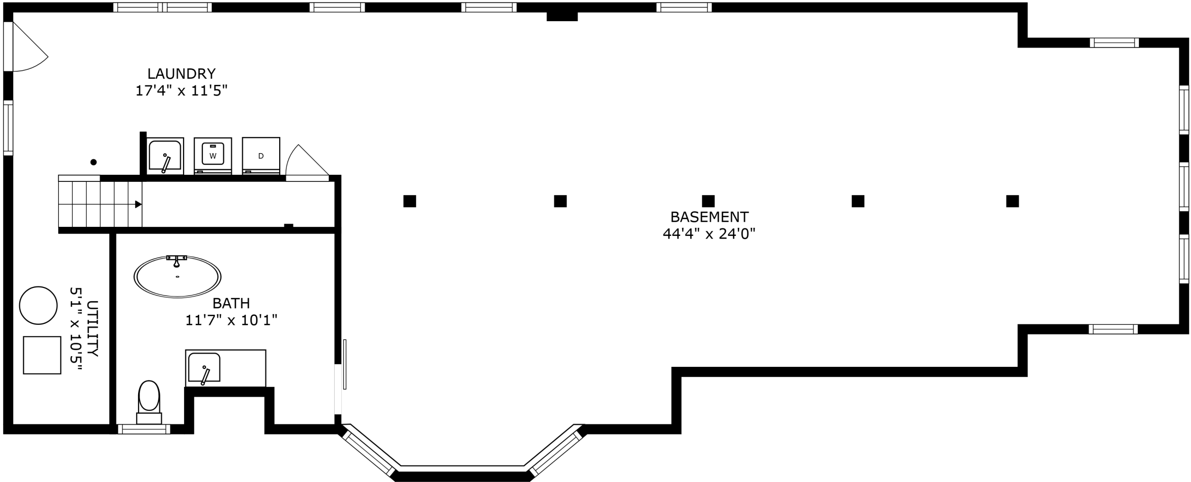
FLOOR 1
