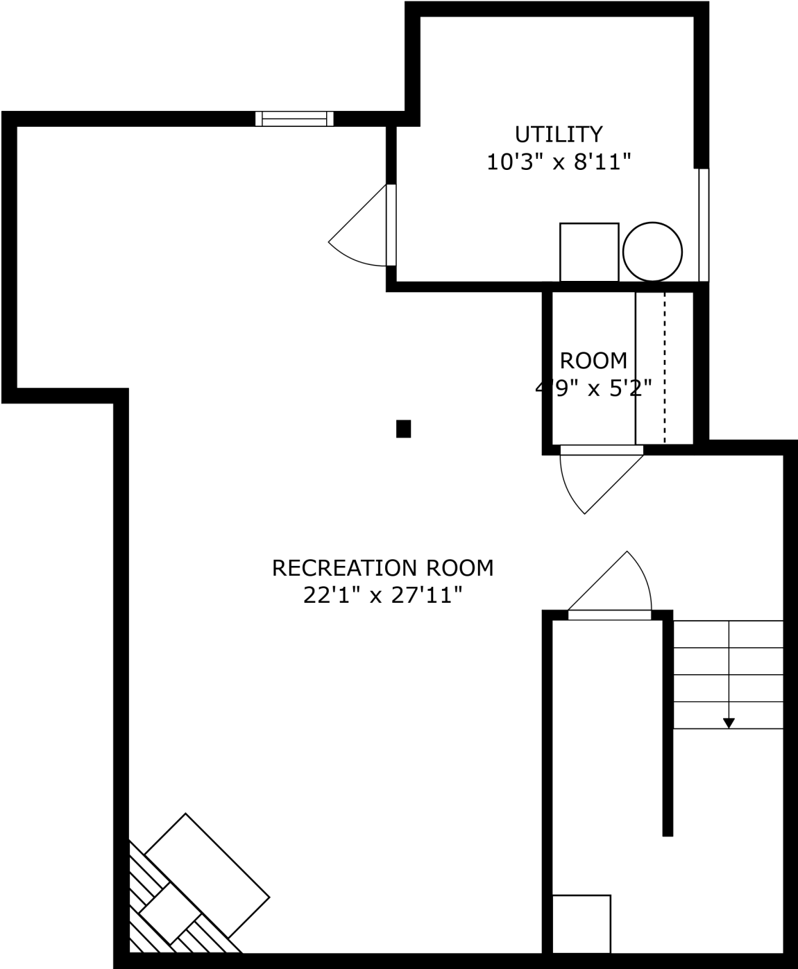
FLOOR 1
