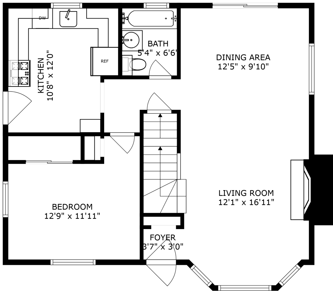
FLOOR 2
