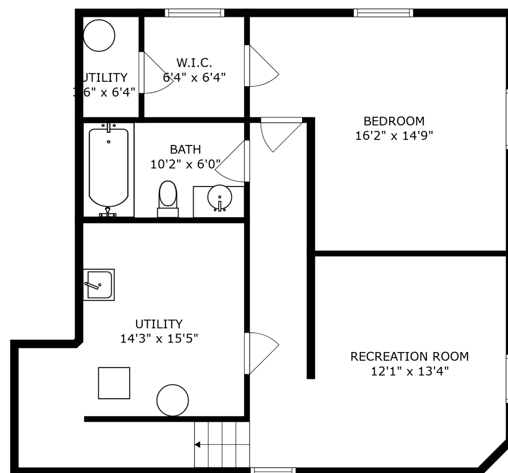
FLOOR 1
