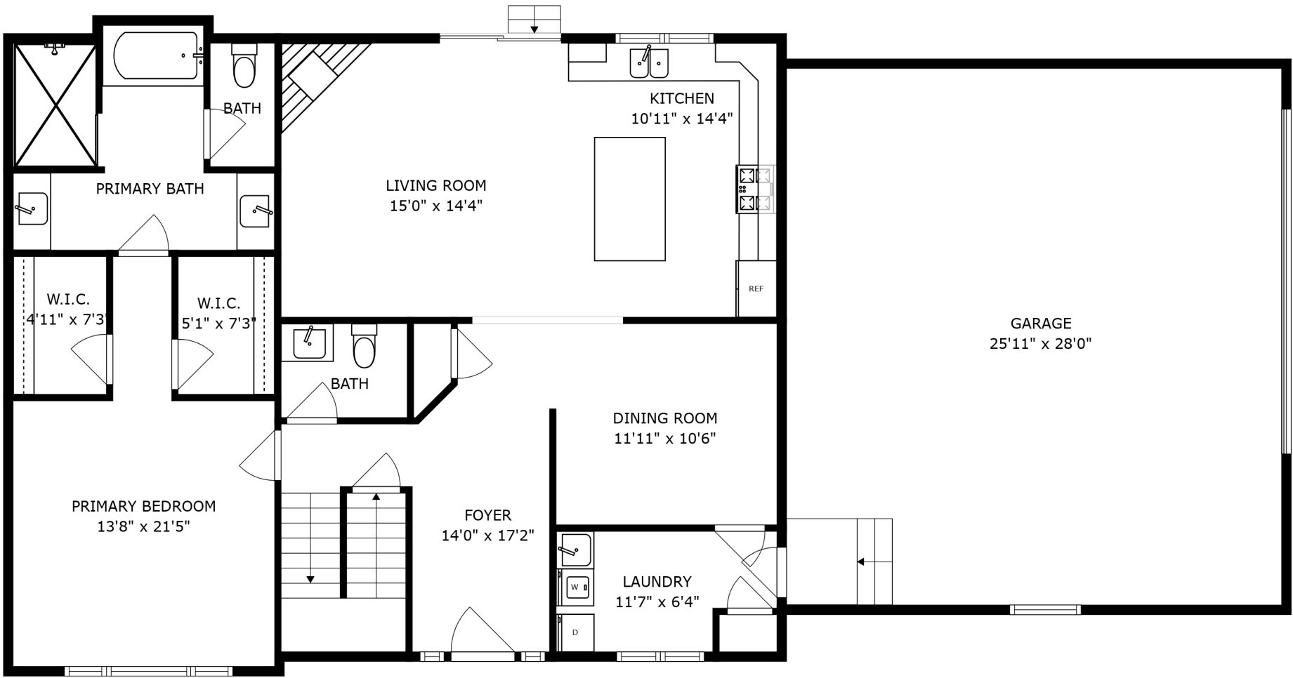
FLOOR 2
