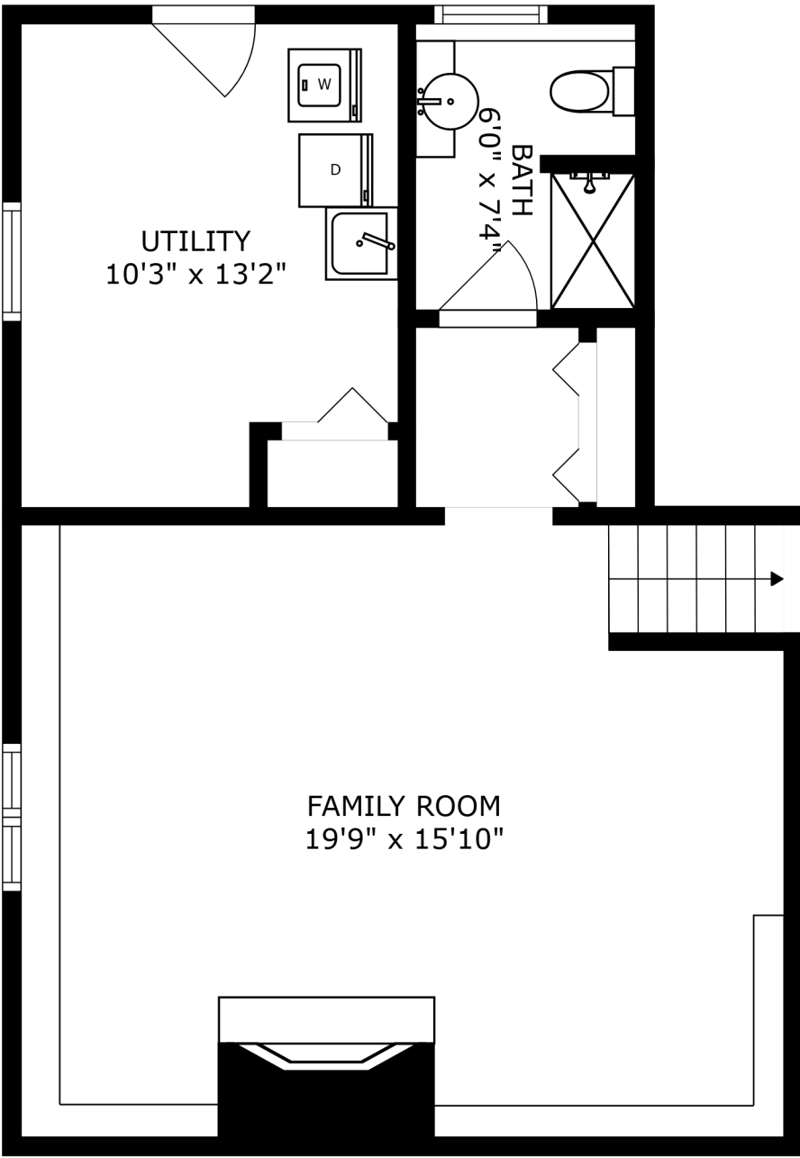
FLOOR 1
