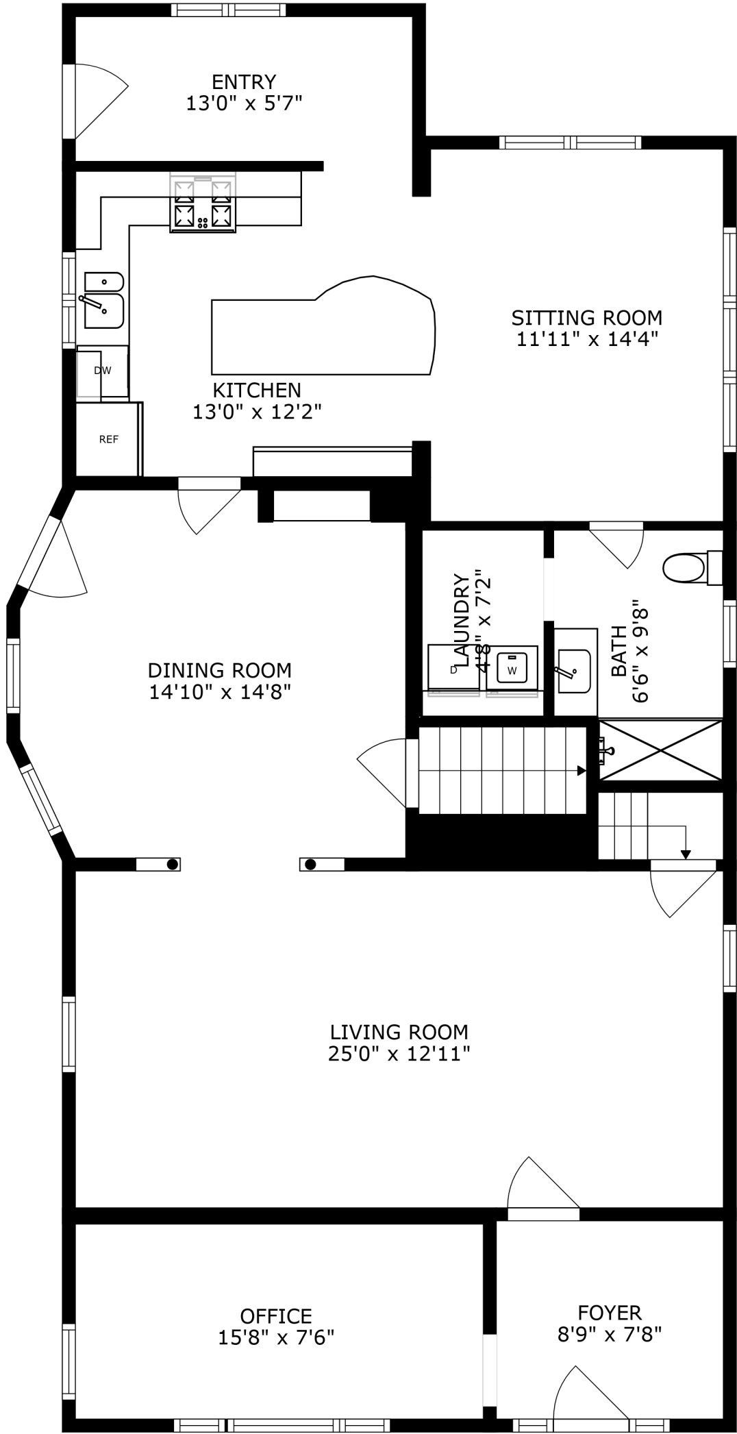
FLOOR 2
