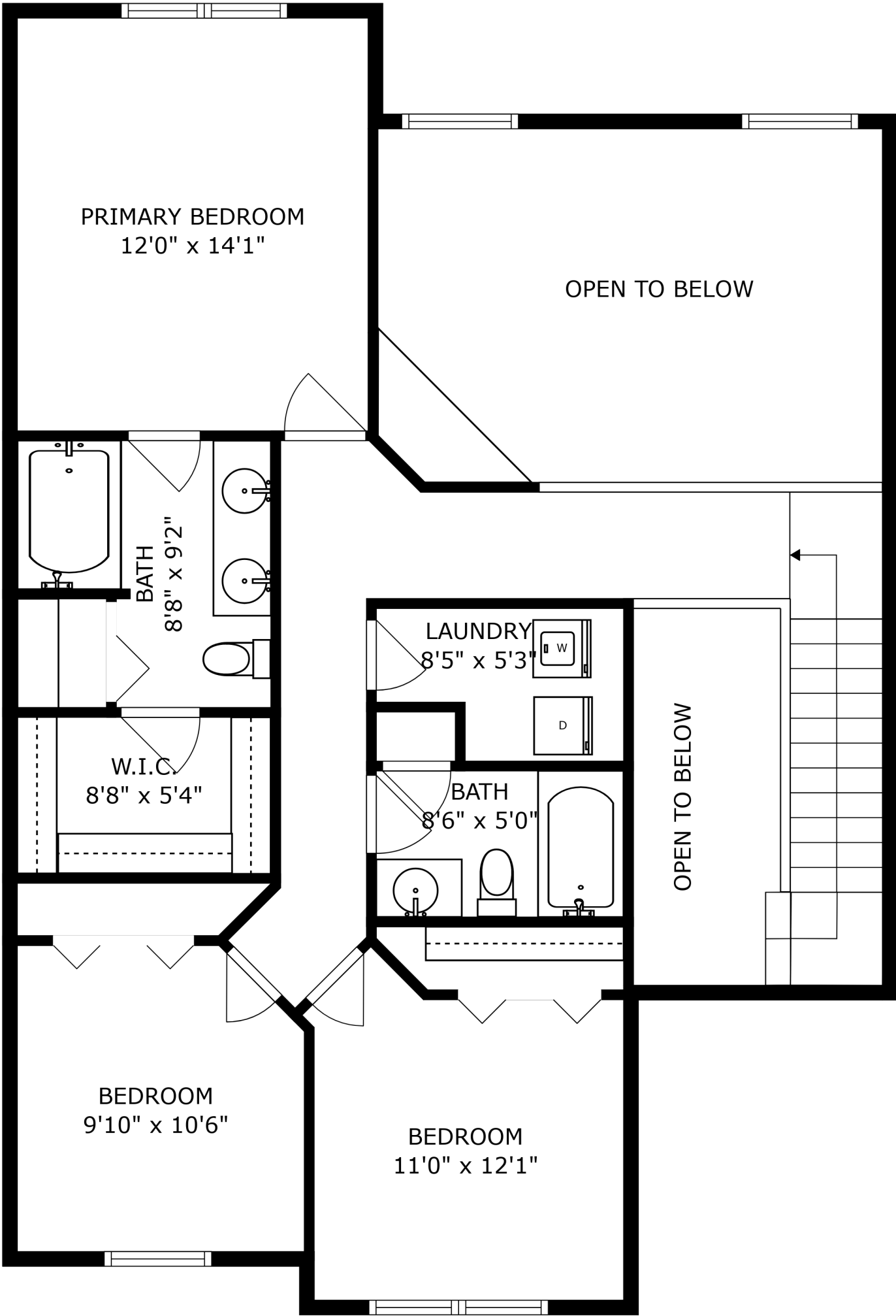
FLOOR 2
