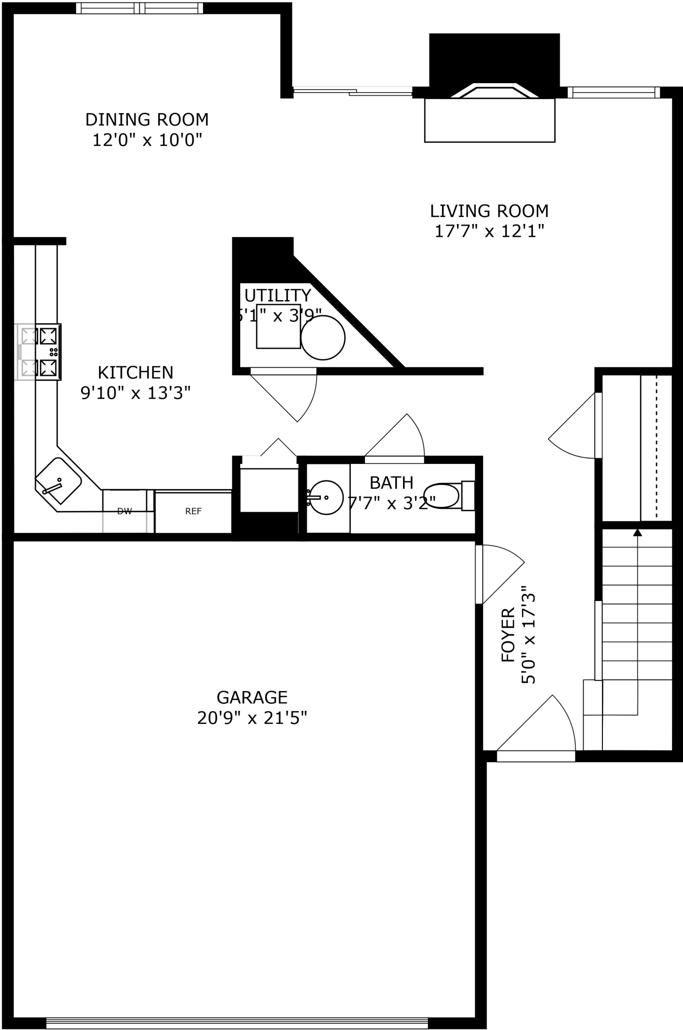
FLOOR 1
