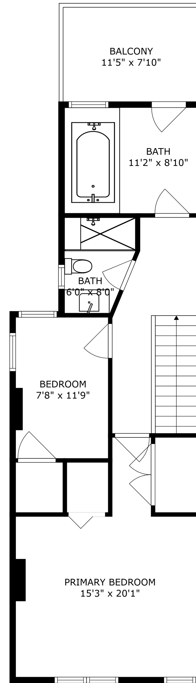
FLOOR 3
