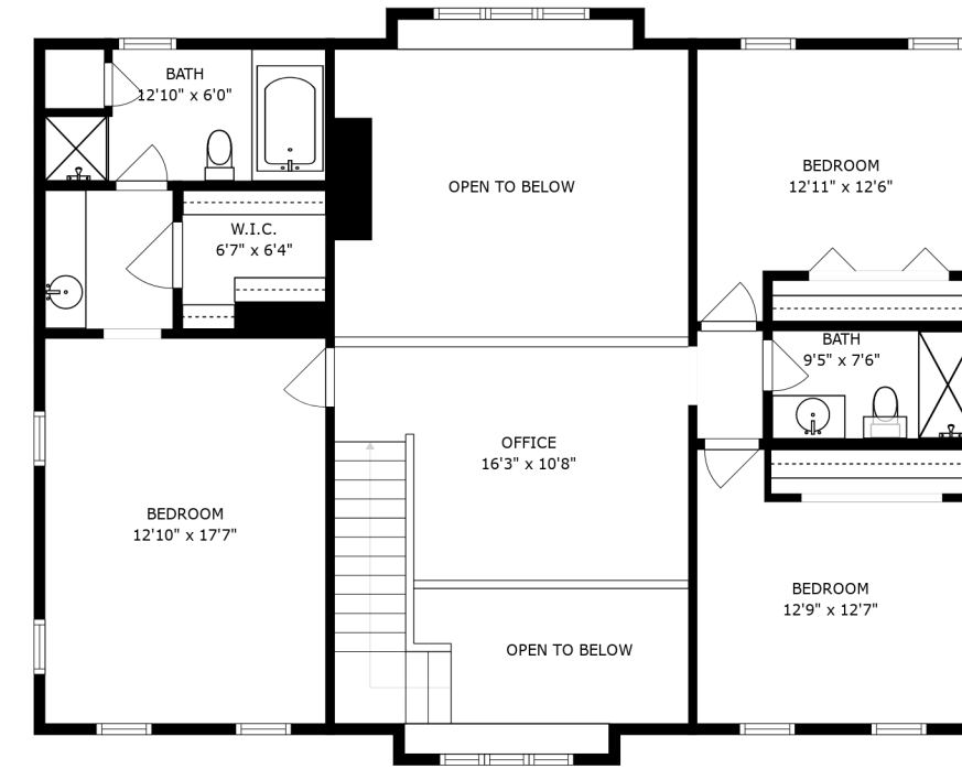
FLOOR 3
