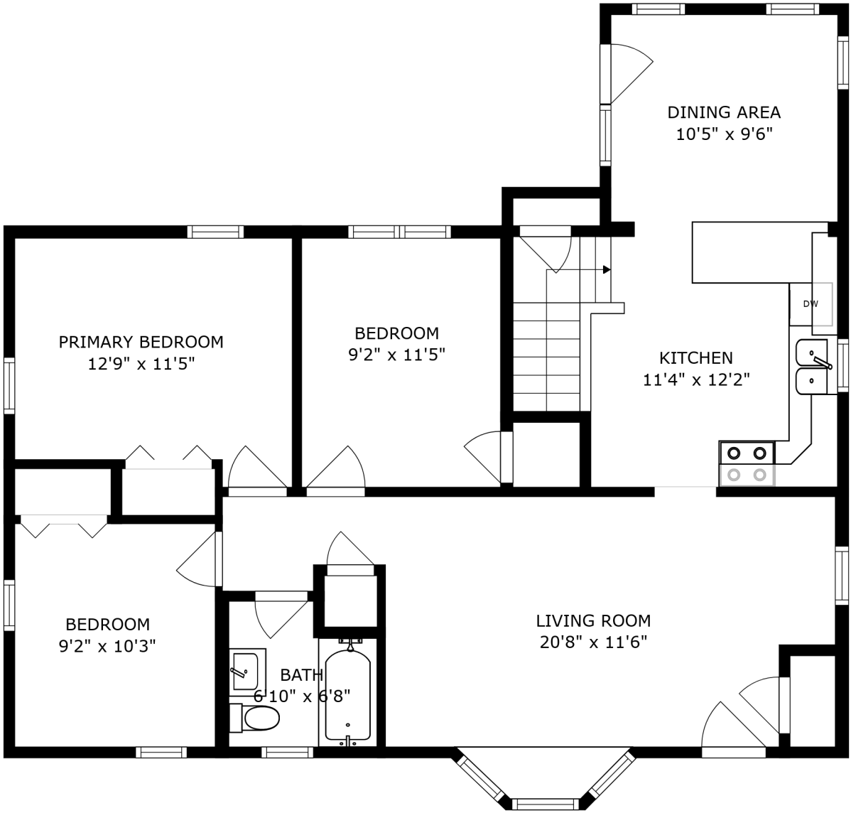
FLOOR 2
