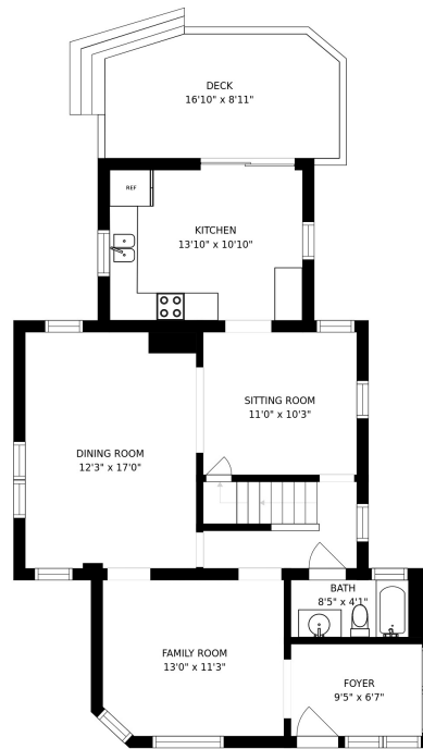
FLOOR 2
