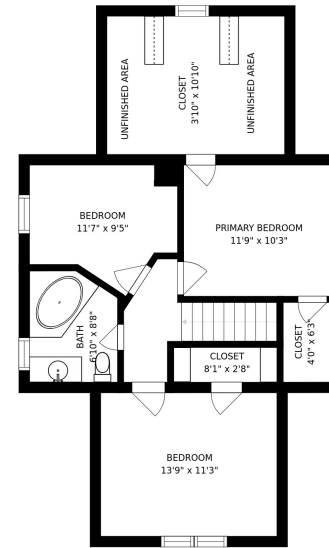
FLOOR 3
