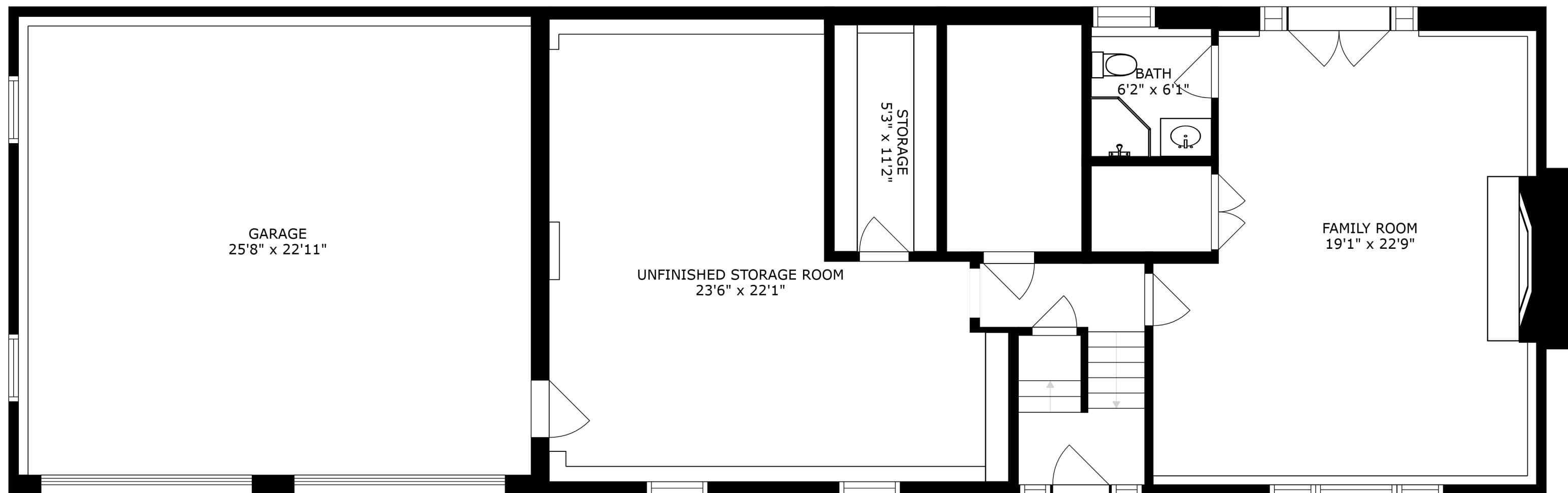
FLOOR 1
