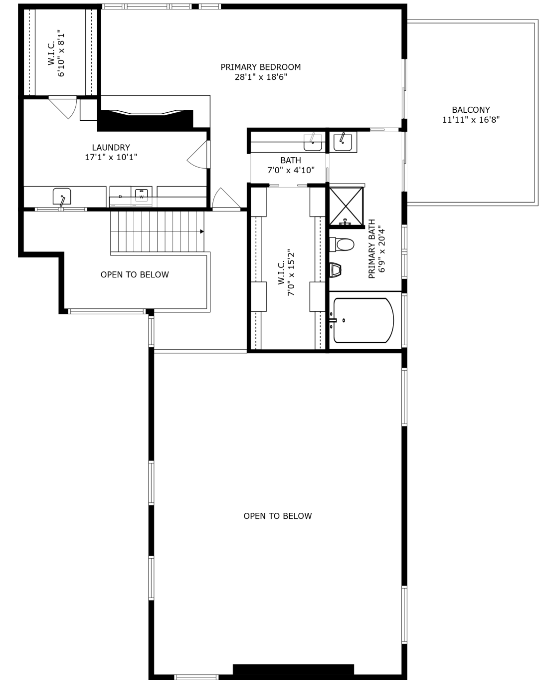
FLOOR 3
