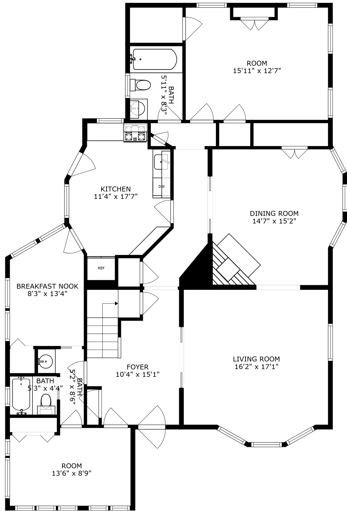
FIRST FLOOR
