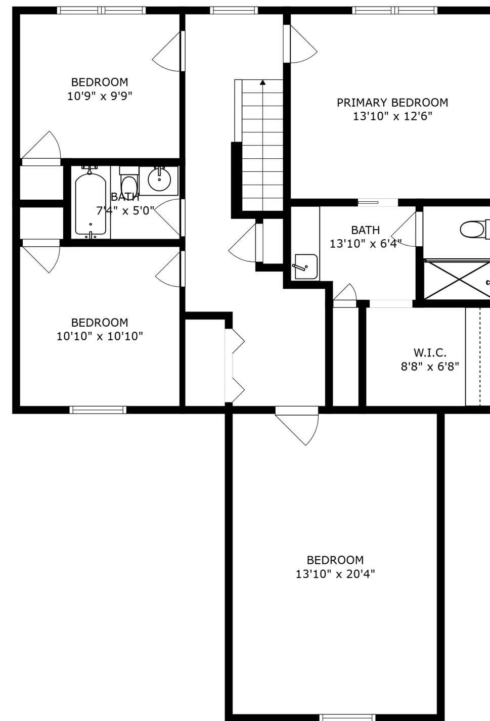
FLOOR 3
