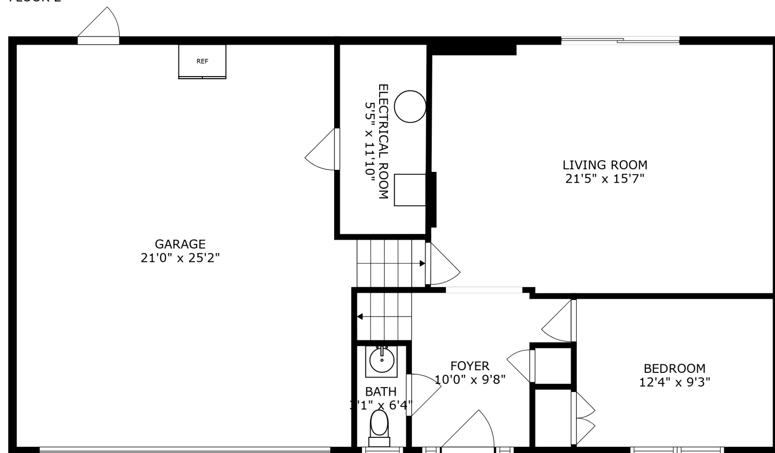
FLOOR 2
