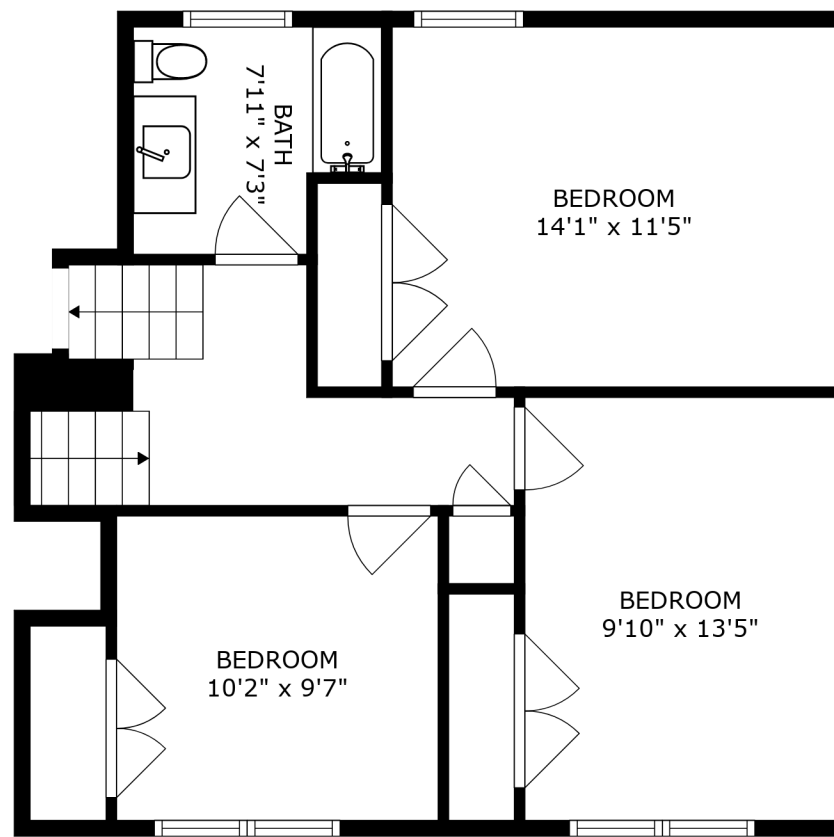
FLOOR 3
