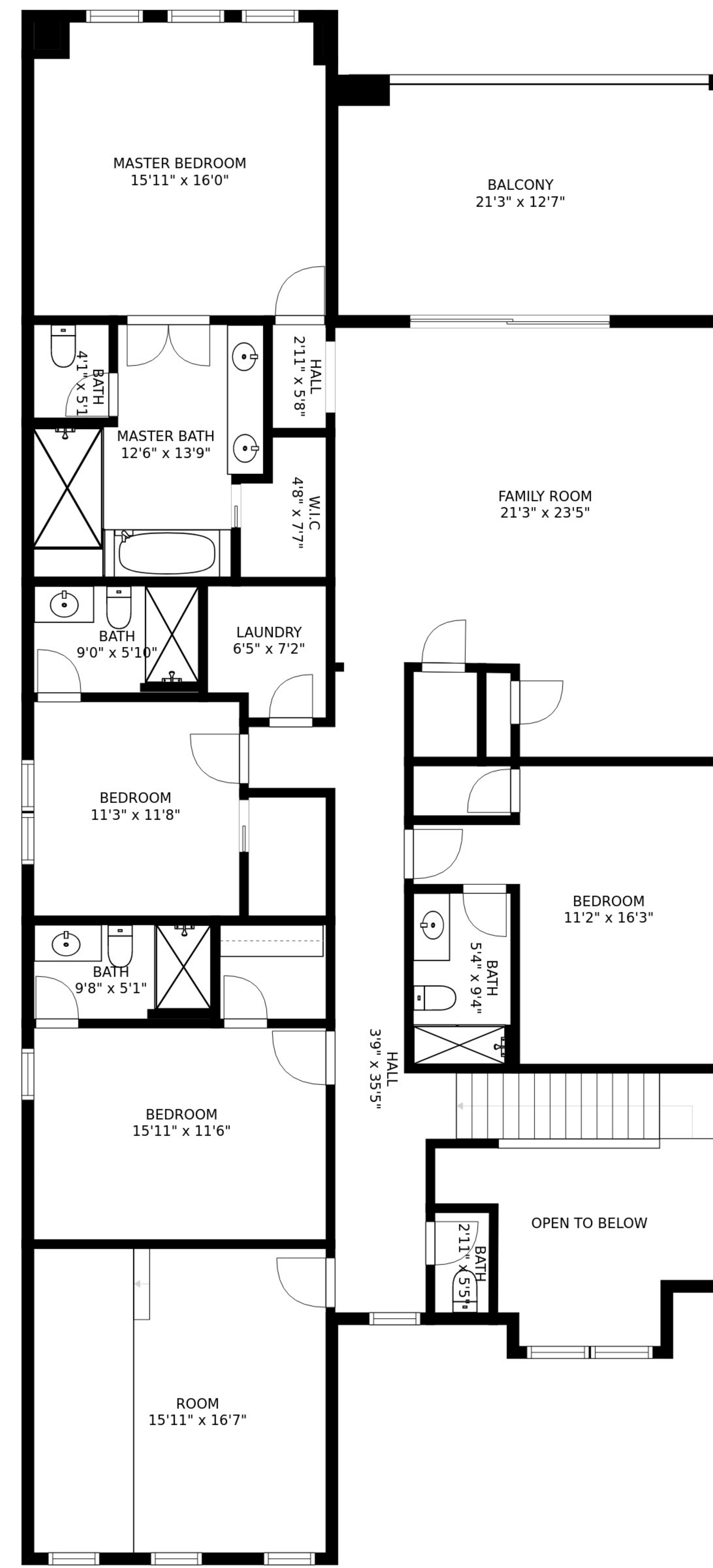
FLOOR 2
