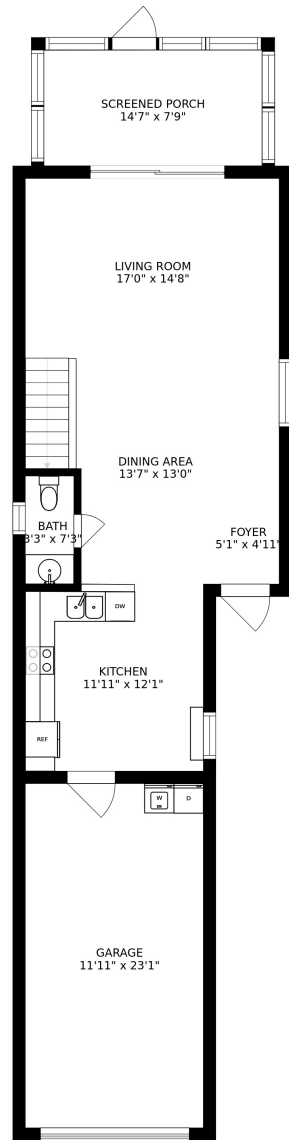
FLOOR 1
