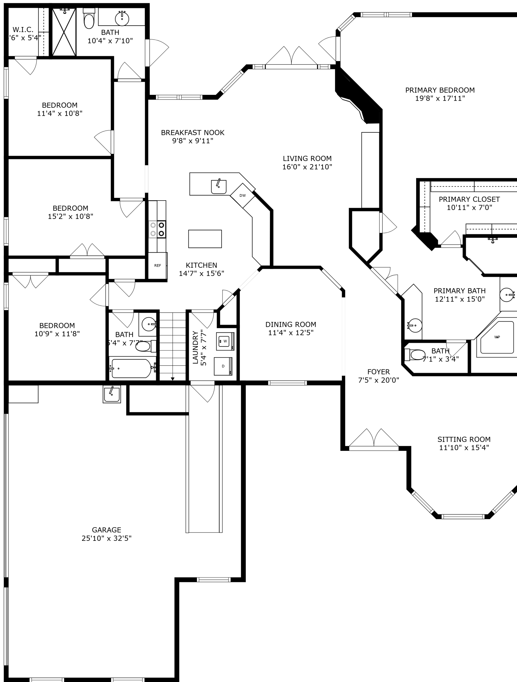
FLOOR 1
