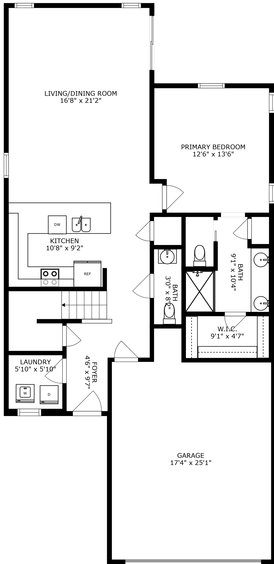
FLOOR 1
