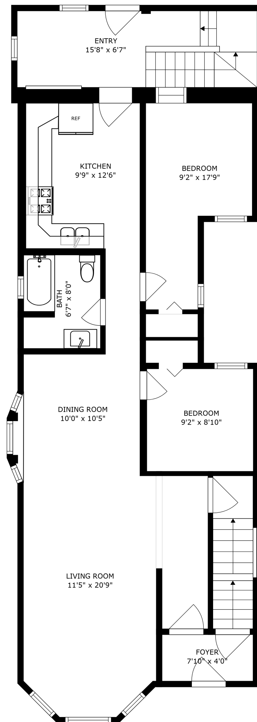
FLOOR 2
