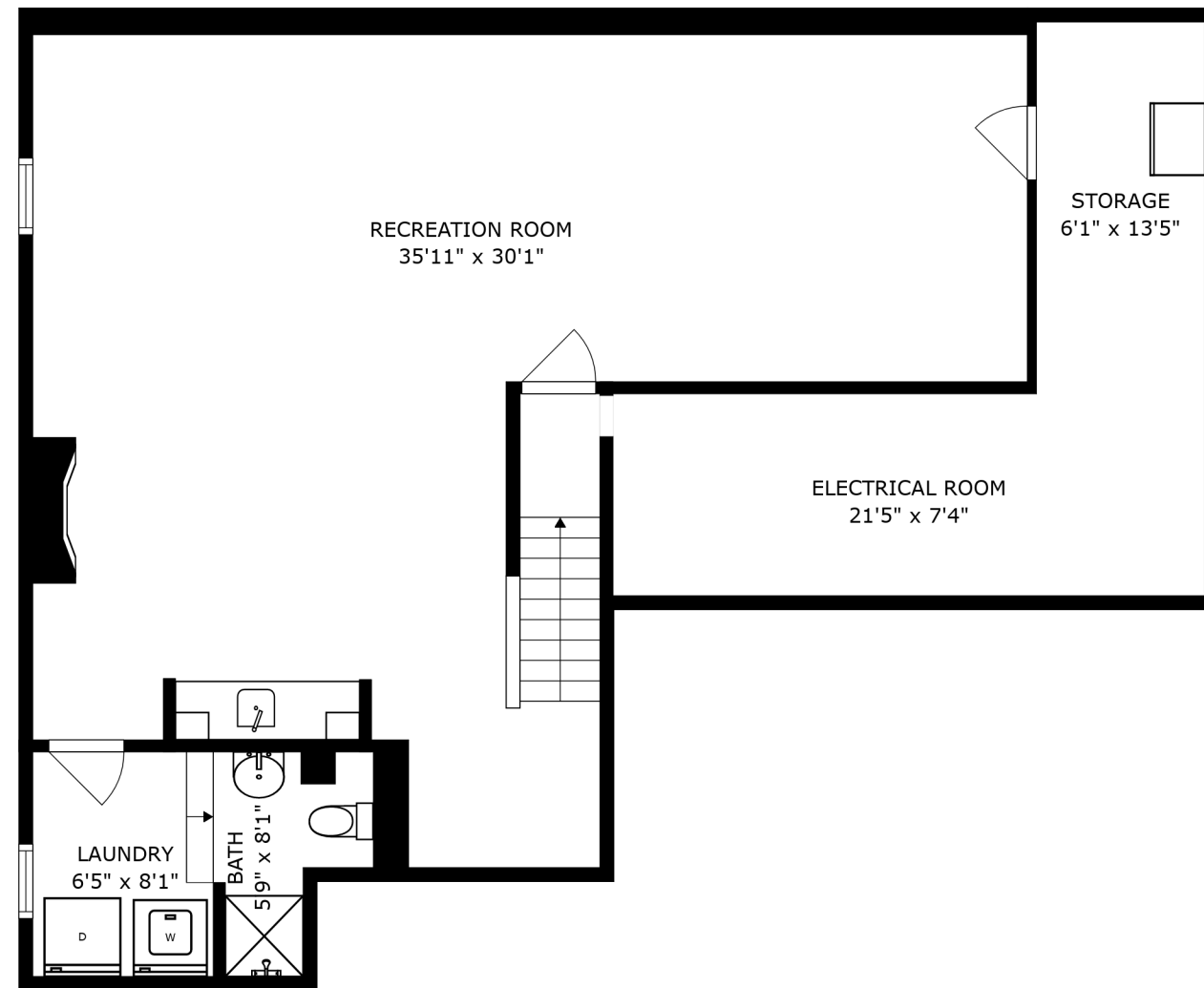
FLOOR 1
