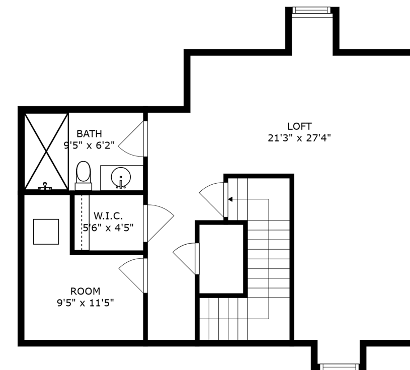
FLOOR 4
