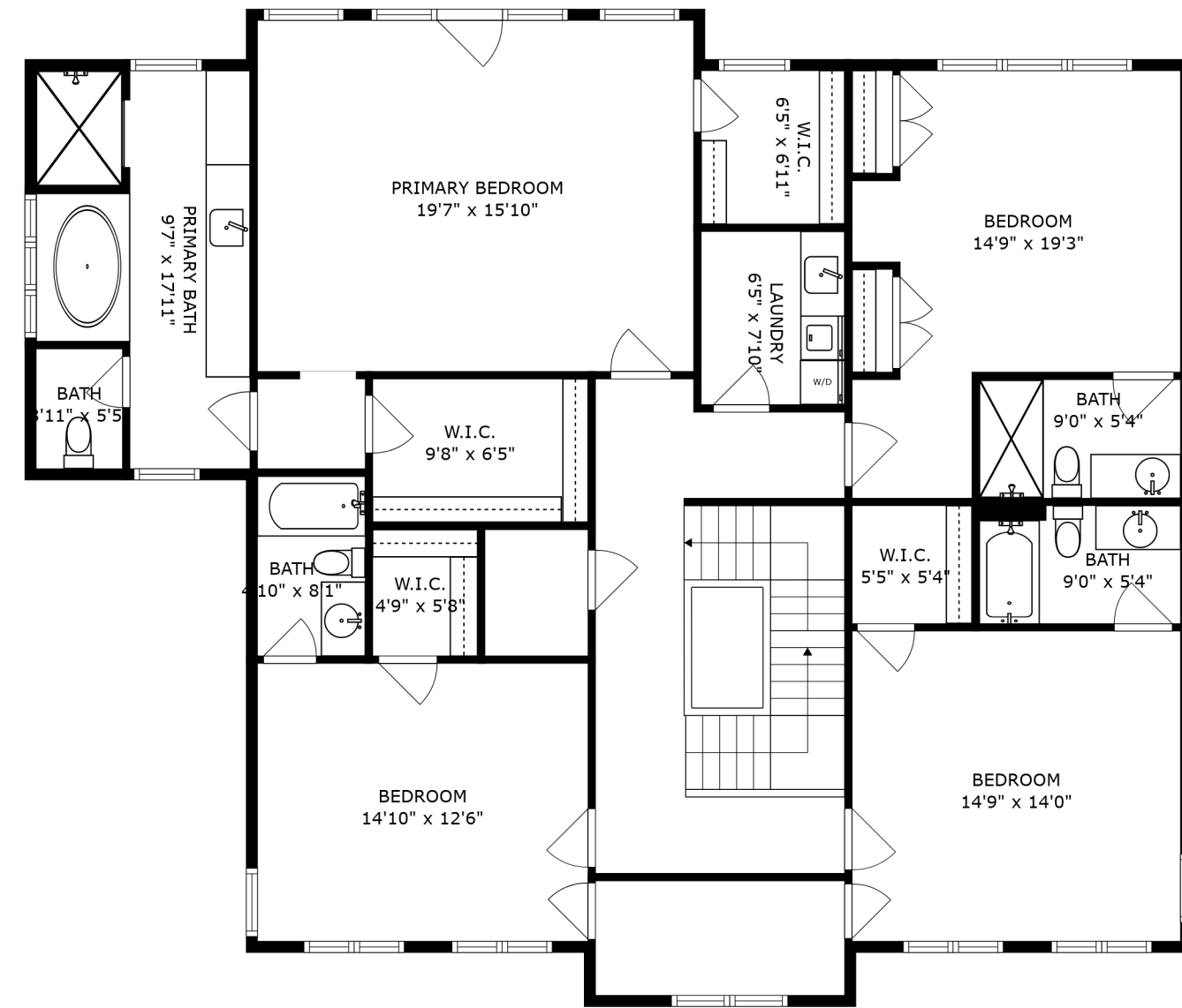
FLOOR 3
