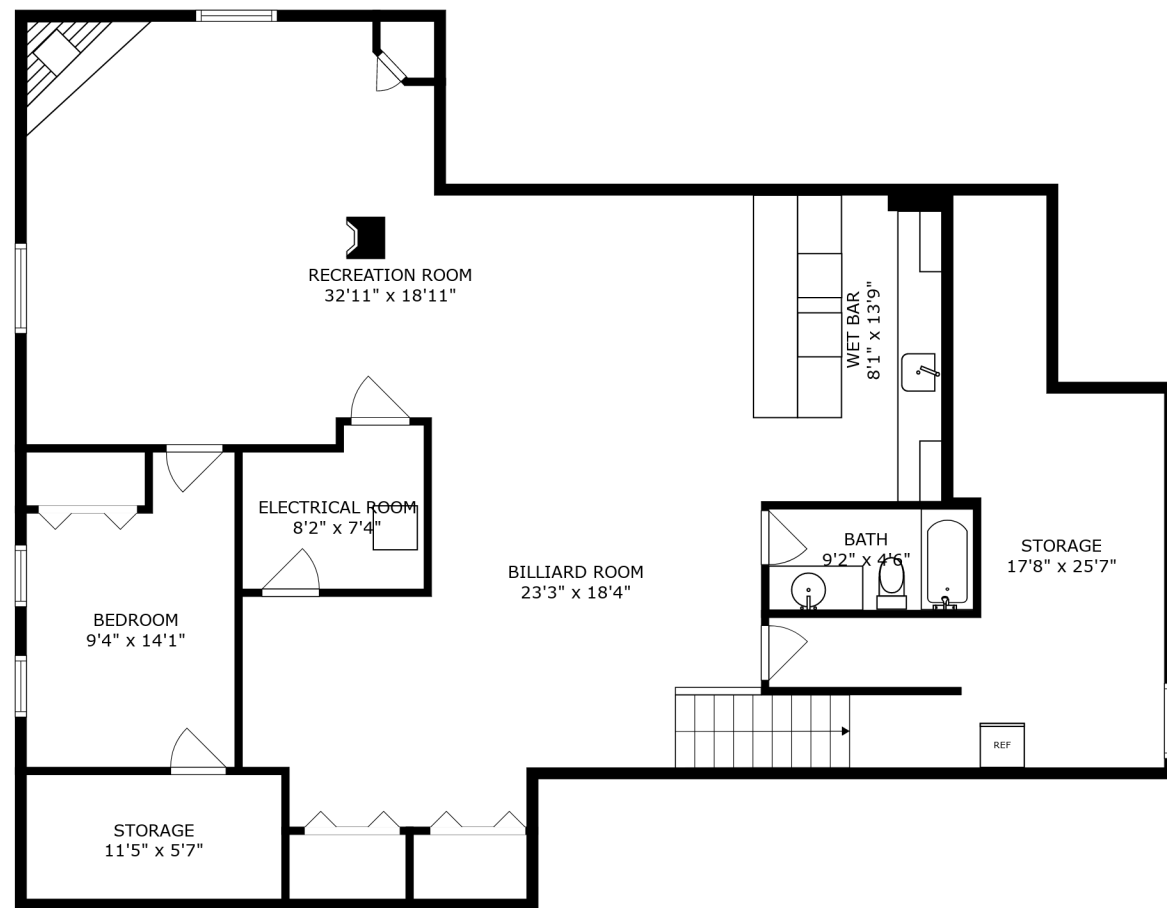
FLOOR 1
