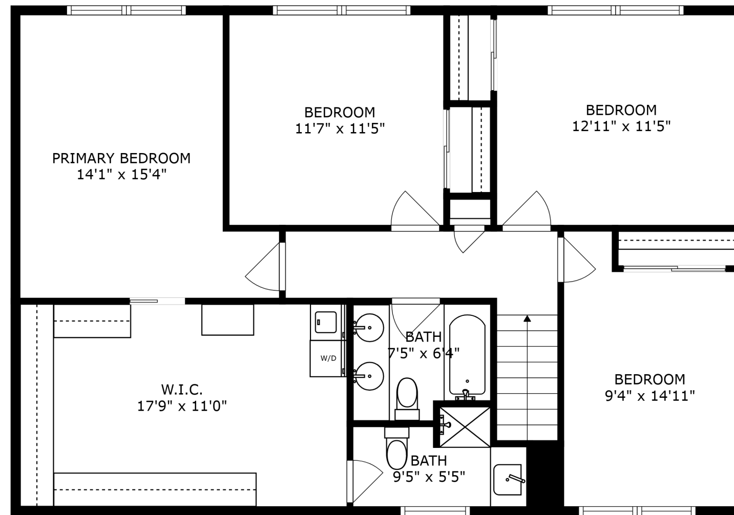
FLOOR 3
