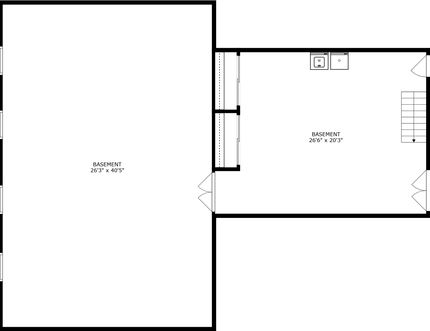
FLOOR 1
