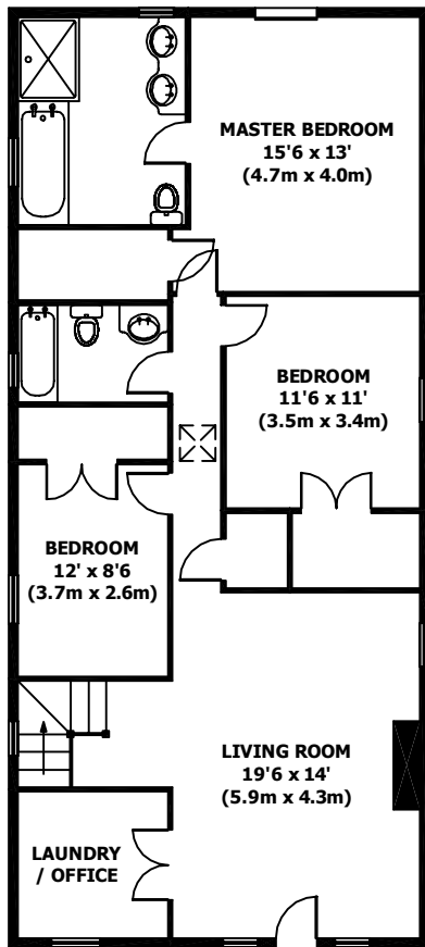
SECOND FLOOR GROSS INTERNAL FLOOR AREA 1176 SQ FT
