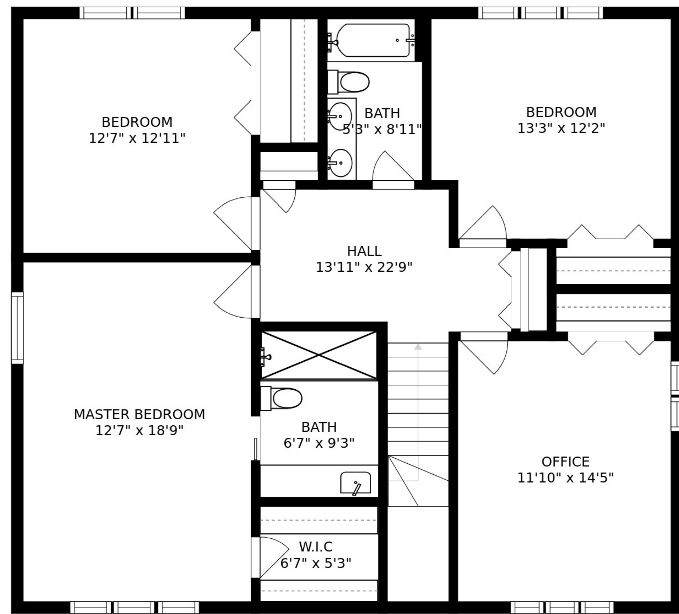
FLOOR 3
